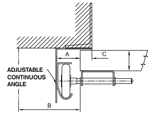
STEEL JAMB OVERLAPPING DOOR
